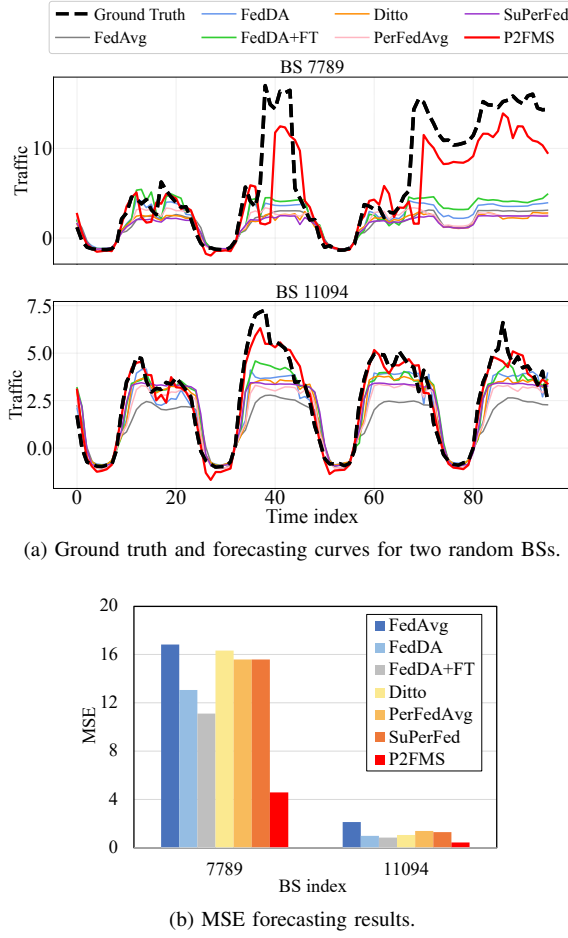
Fig. 2: Prediction result comparisons of different FL methods.
