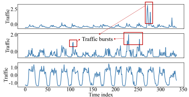
Fig. 1: Traffic data of different BSs in Trentino.
