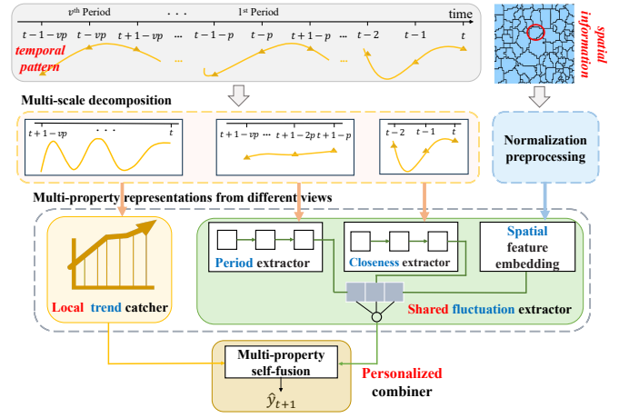
Fig. 4: The structure of client-side customized model.
