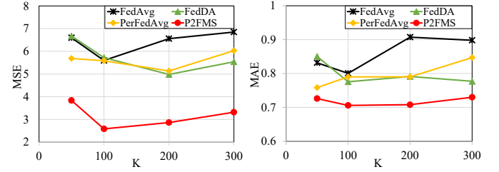
Fig. 9: MSE and MAE results under different client numbers.
