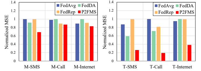
Fig. 10: Generalization evaluations for new clients.
