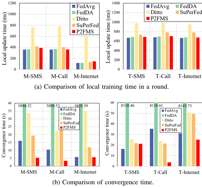
Fig. 11: Running time analysis.
