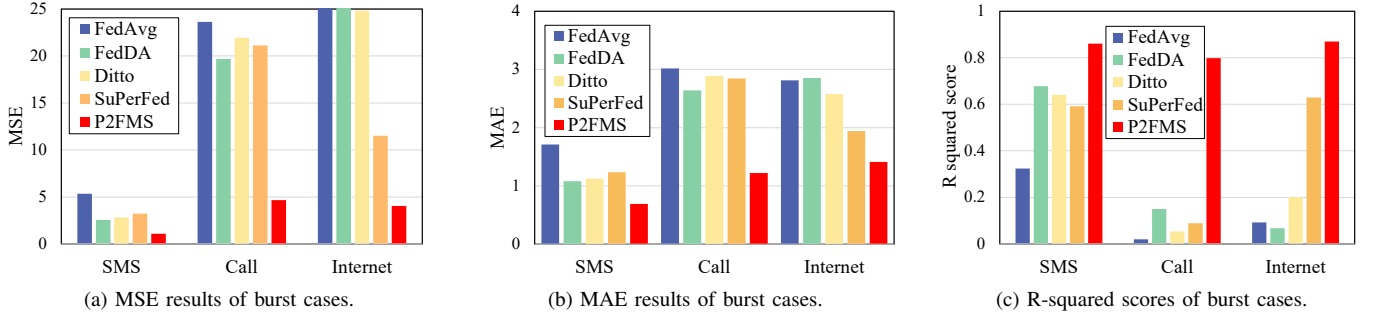
Fig. 6: Performance evaluations on burst cases of Trentino.
